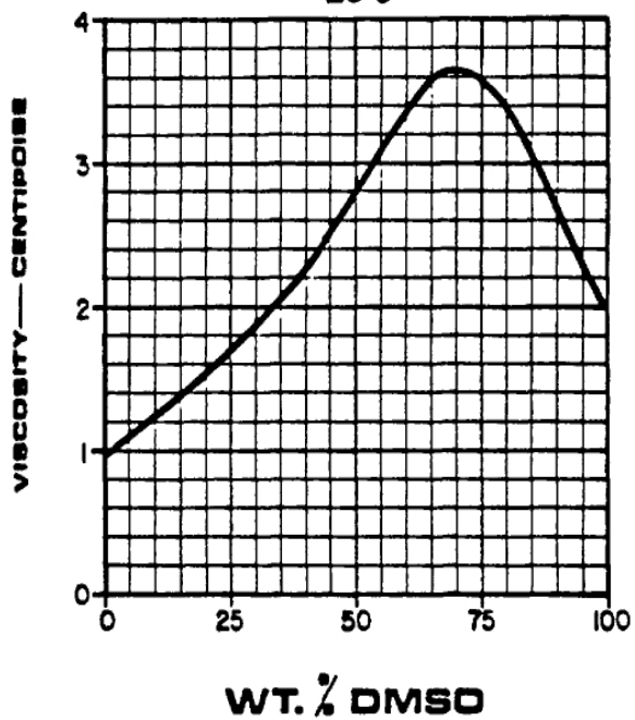
FIGURE 4 VISCOSITY OF DMSO-WATER SOLUTIONS 25°C
