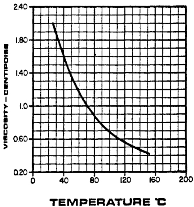
FIGURE 3 VISCOSITY OF DMSO
