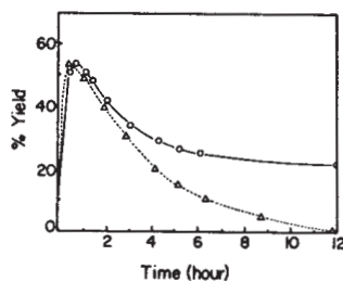
Figure 6. Product formation vs. time and effect of copper(II): \text{O} , without \text{Cu}(\text{OAc})_2 ; \Delta , with \text{Cu}(\text{OAc})_2 .
