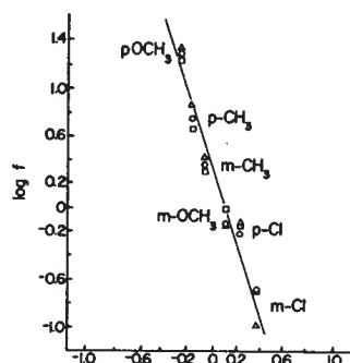
Figure 8. Hammett treatment using \sigma value.
