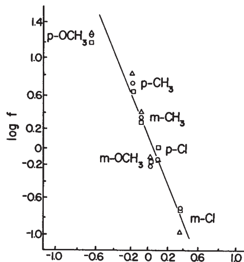
Figure 9. Hammett treatment using \sigma^+ value.
