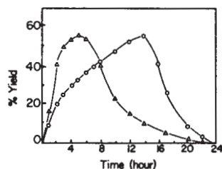
Figure 4. Effect of copper(II) on nitromethylation rate: \Delta , with \text{Cu}(\text{OAc})_2 ; \text{O} , without \text{Cu}(\text{OAc})_2 .
