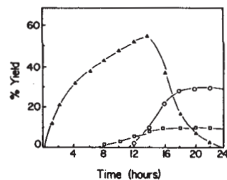
Figure 1. Product formation vs. time for CAN-C 6 H 6 -CH 3 NO 2 : \Delta , C 6 H 5 CH 2 NO 2 ; \circ , C 6 H 5 CHO; \square , C 6 H 5 CH 2 OAc.
