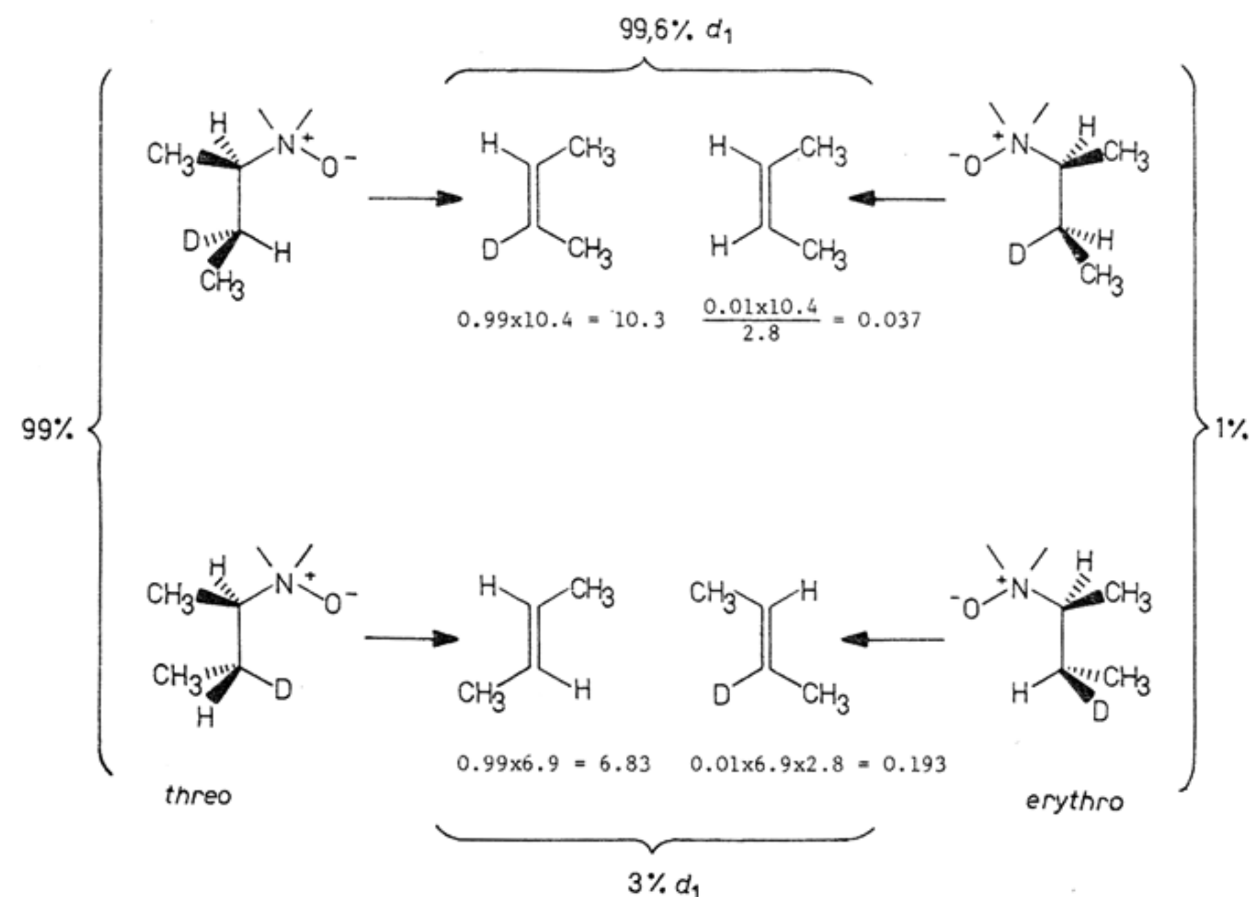
SCHEME 1. DECOMPOSITION OF THE AMINE OXIDE OBTAINED FROM cis -2-BUTENE
