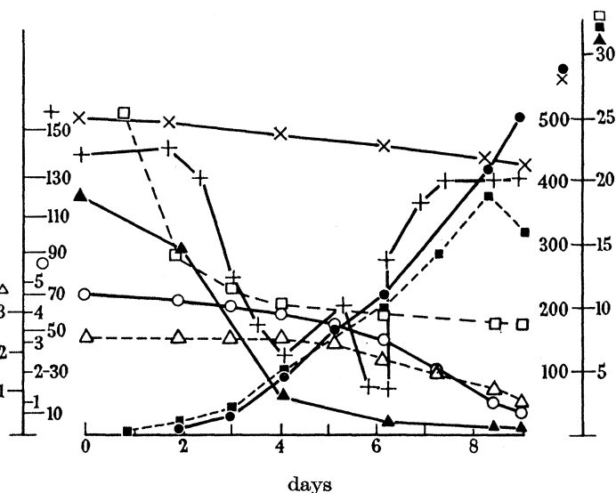
FIGURE 9. Course of a typical LAD fermentation by Claviceps paspali , strain F-550, in a 500 l. stirred fermenter in medium B. \Delta , Succinic acid, g%; \circ , mannitol, g%; \square , Q_{o_2} ; \blacksquare , dry weight, mg/ml.; \blacktriangle , inorganic phosphate, mg P%; \bullet , LAD , \mu g/ml.; \times ammonia, mg N%; +, dissolved oxygen, per cent saturation at 1 atm over-pressure of air.
