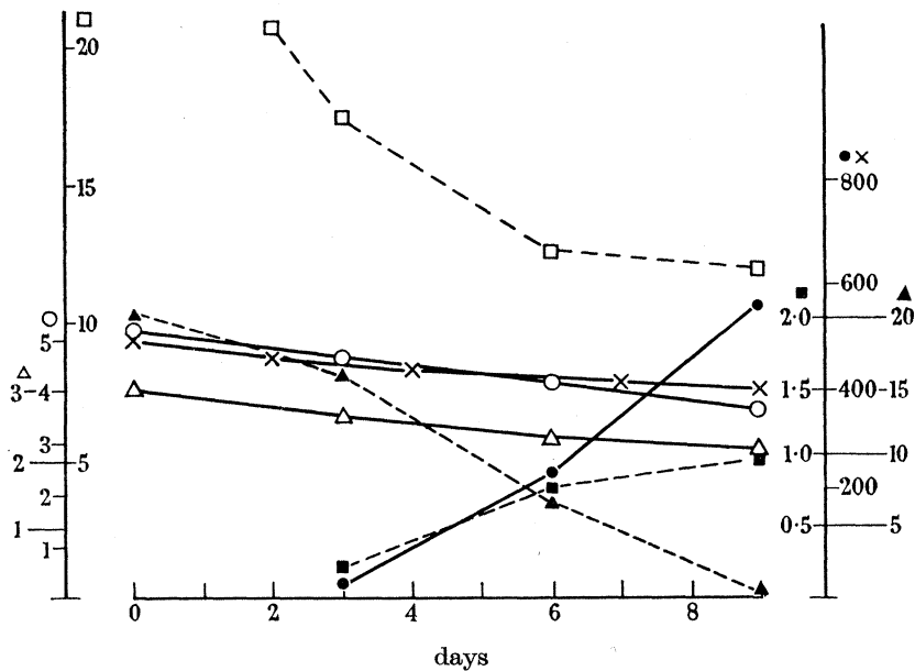
FIGURE 8. Course of a typical LAD fermentation by Claviceps paspali , strain F-550, in shake flasks in medium B. \Delta , Succinic acid, g%; \circ , mannitol, g%; \square , Q_{o_2} ; \blacksquare , dry weight, g/100 ml.; \blacktriangle , inorganic phosphate, mg P%; \bullet , LAD \mu g/ml.; \times , ammonia, mg N%.
