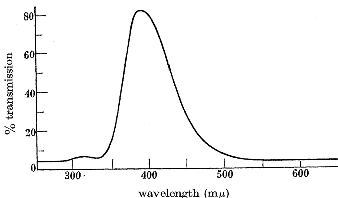
FIGURE 15. Ultra-violet fluorescence spectrum of B_1 . ( c 5 \mu\text{g}/\text{ml} . in 95% ethanol; exciting wavelength 320 \text{m}\mu .)
